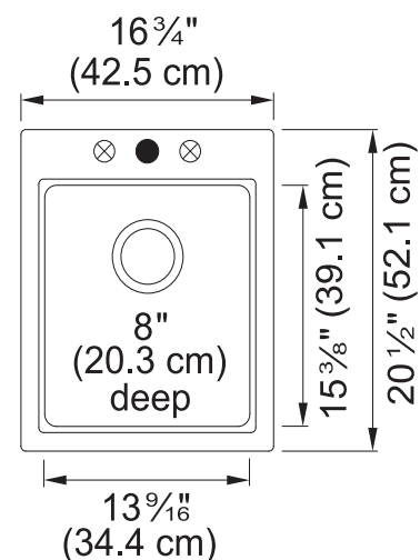
Dimensional Drawing
